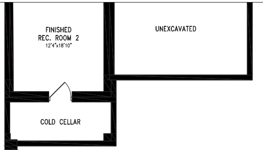
PARTIAL OPTIONAL FINISHED BASEMENT PLAN ELEV. 'B'
